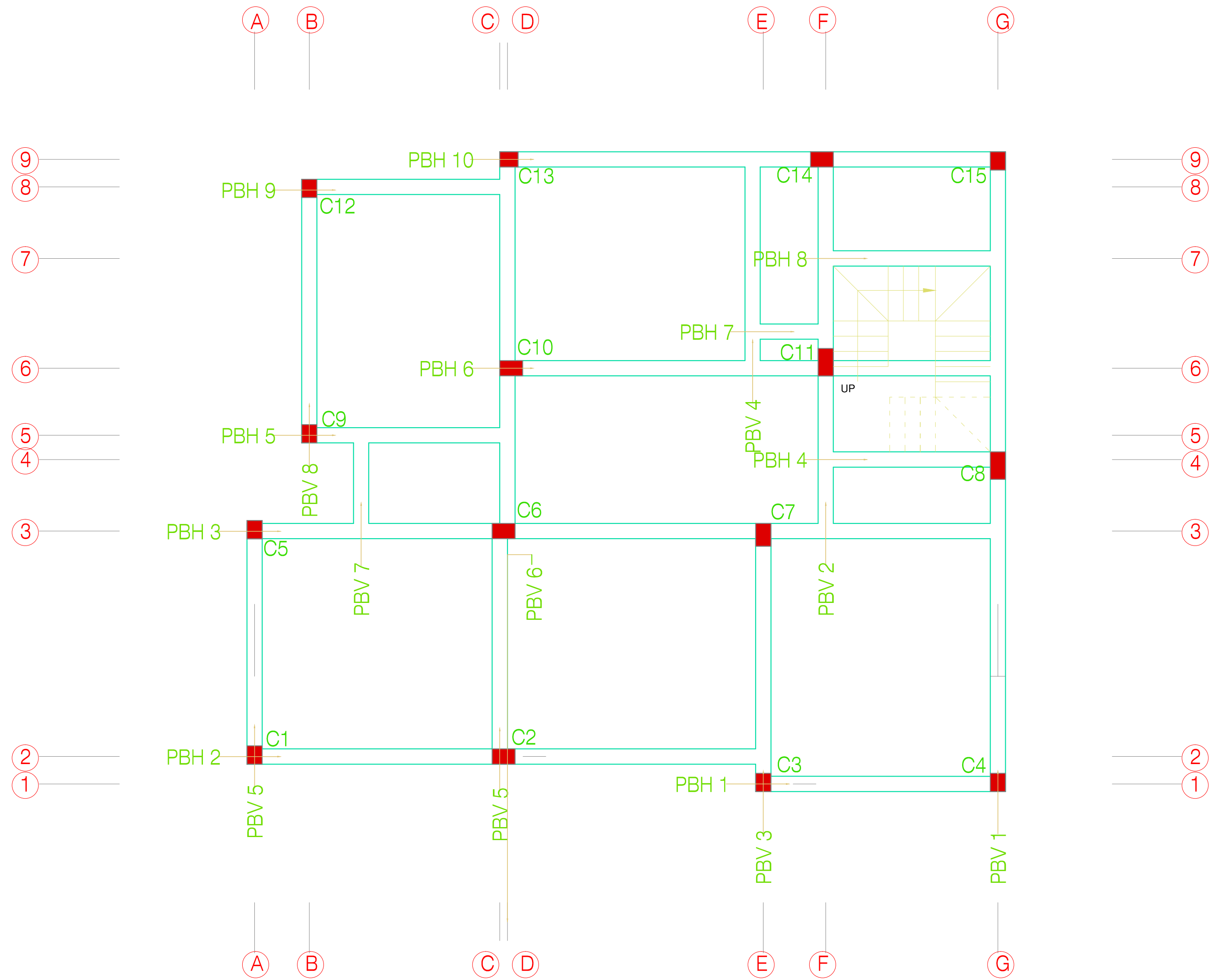
MARKING PLAN OF PLINTH BEAM
