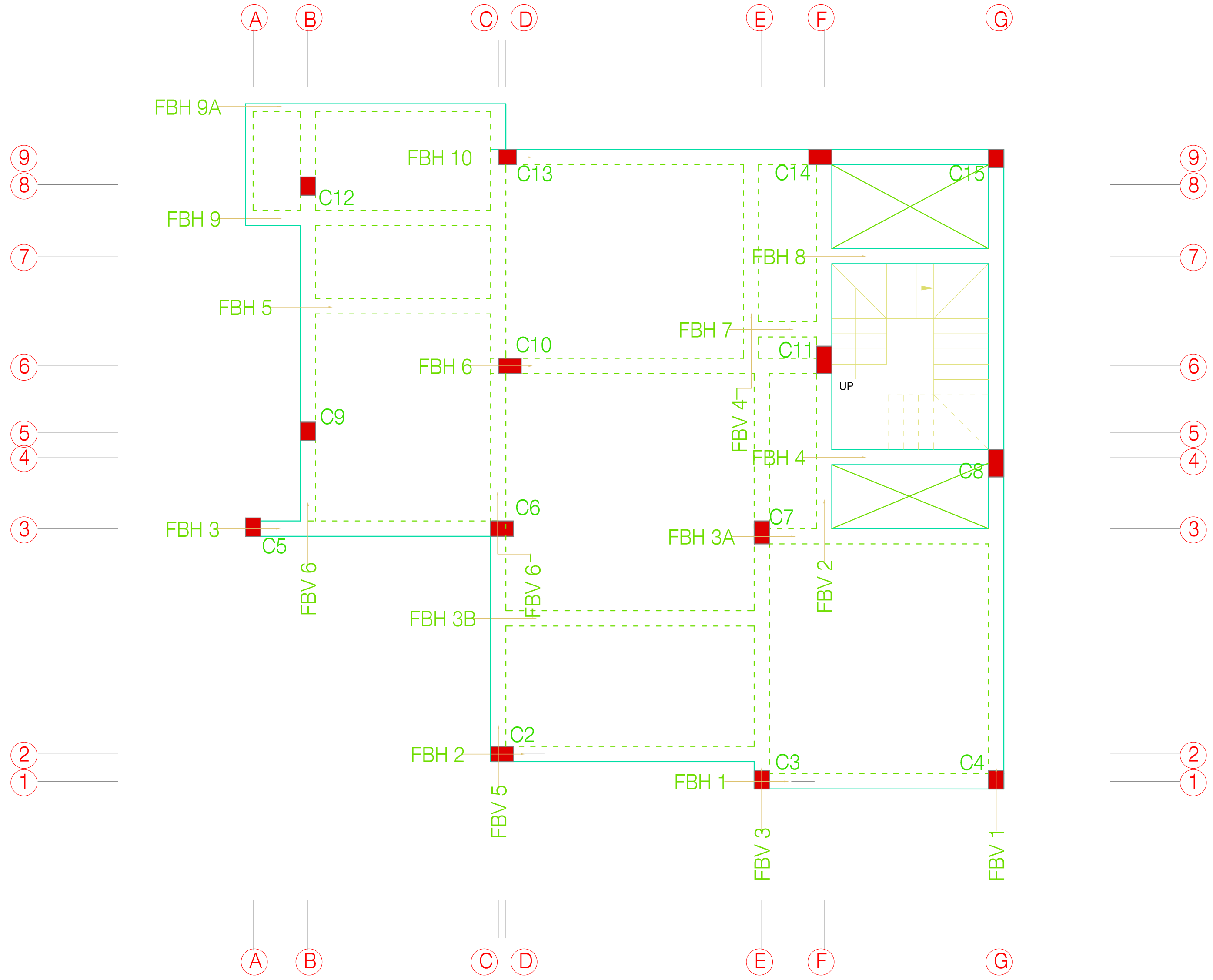
MARKING PLAN OF 1 ^ ST. FLOOR ROOF BEAM
