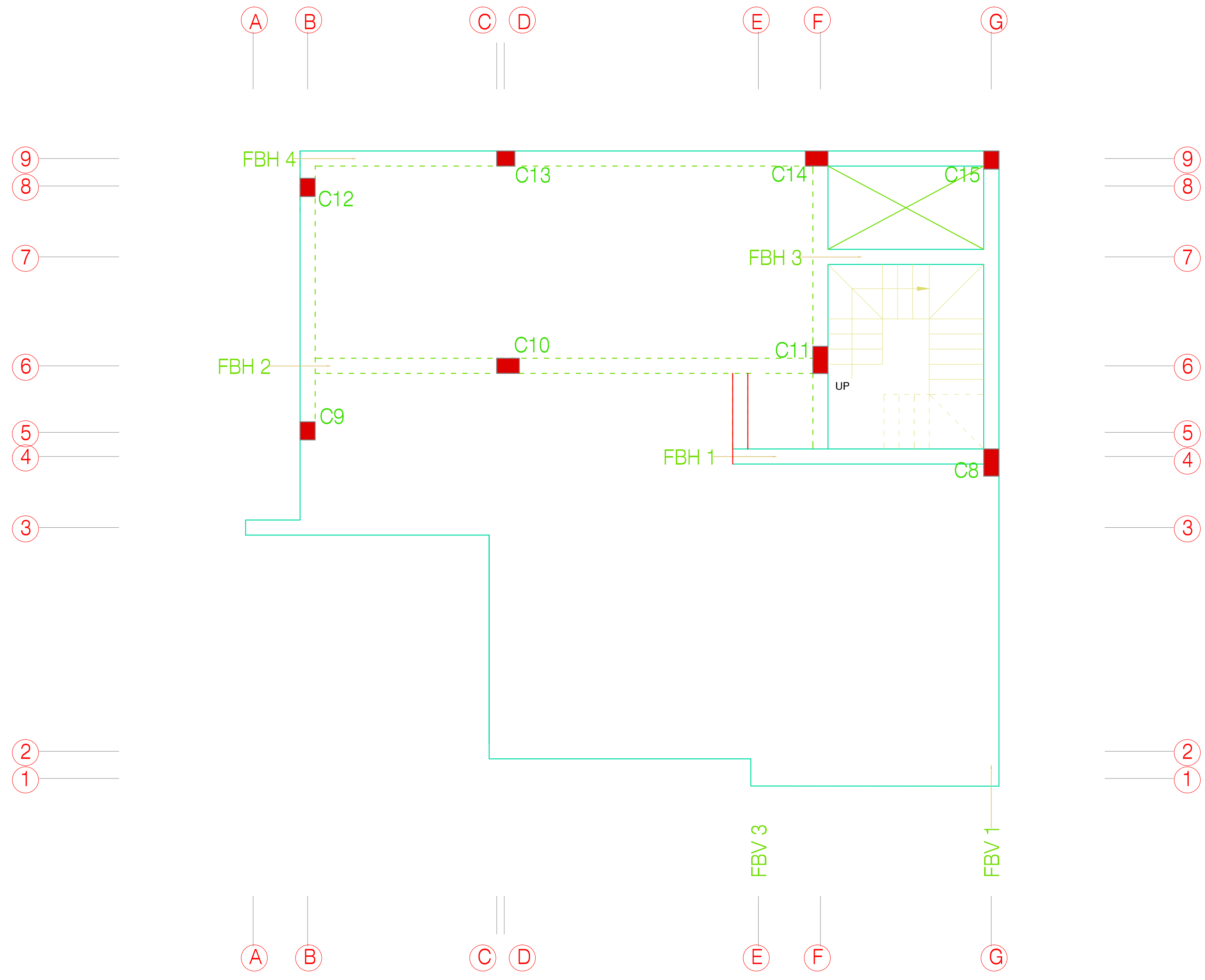
MARKING PLAN OF 2 ND . FLOOR ROOF BEAM
