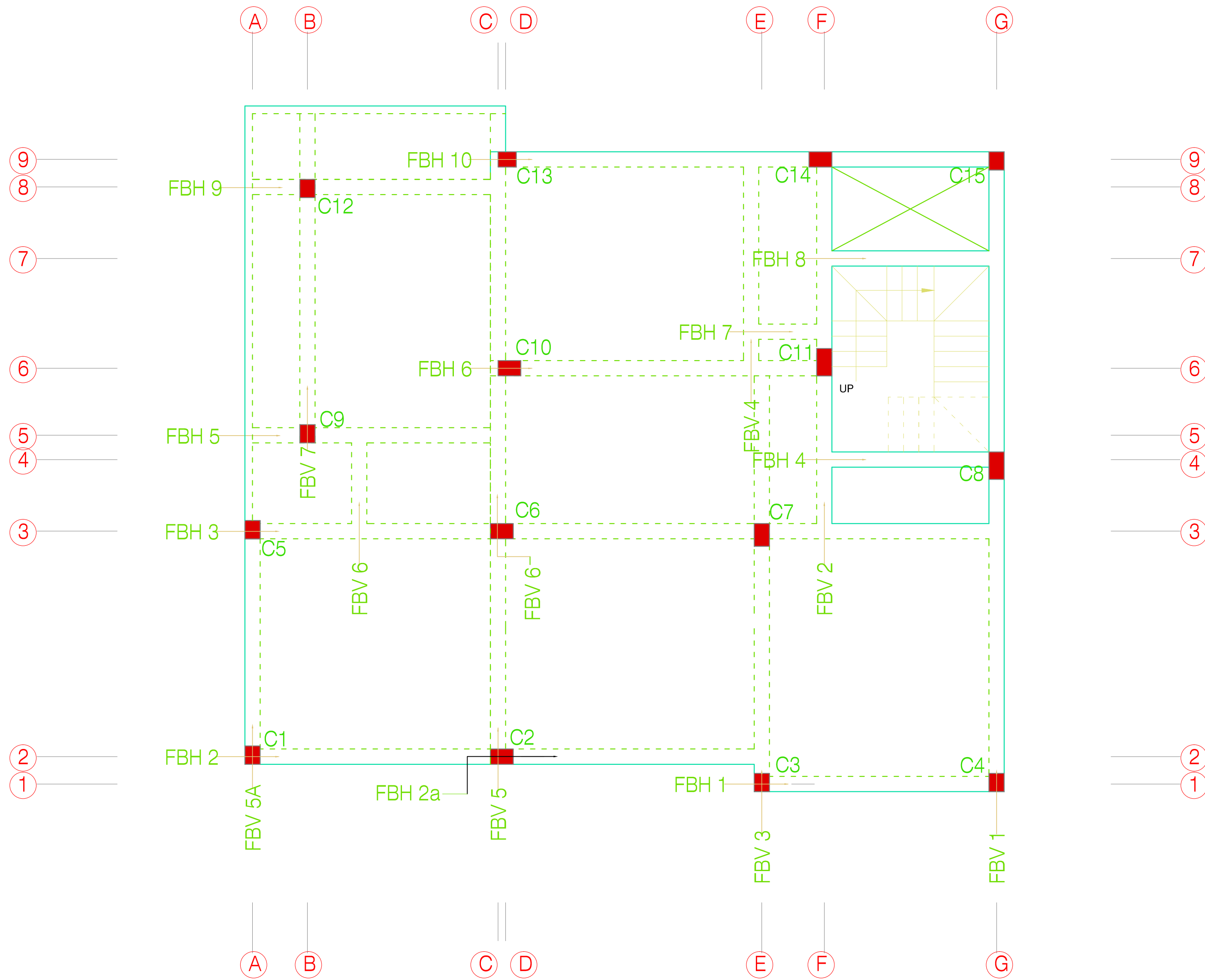
MARKING PLAN OF GR. FLOOR ROOF BEAM
