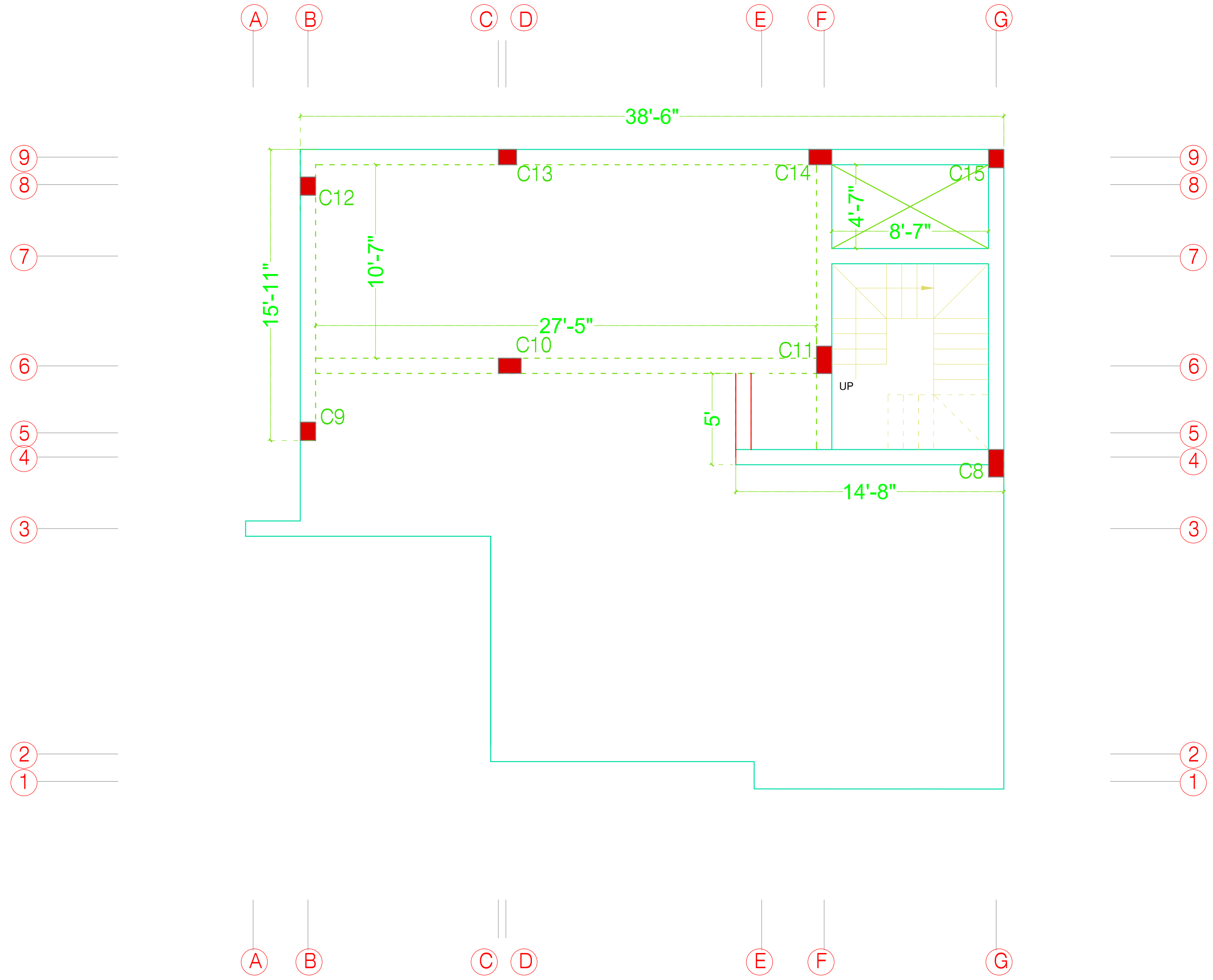
SHUTTERING PLAN OF 2 ND . FLOOR ROOF BEAM
