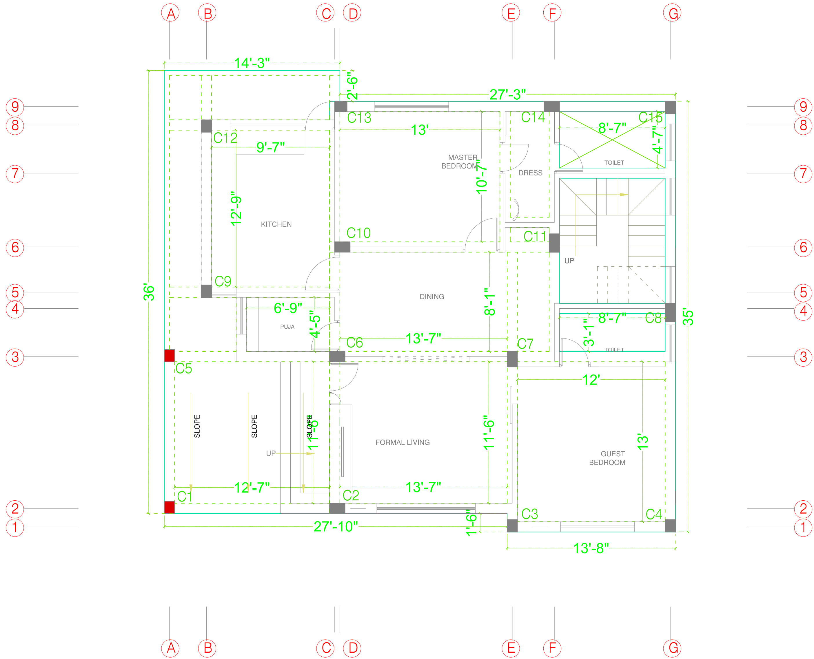
SHUTTERING PLAN OF GR. FLOOR ROOF BEAM
